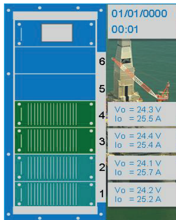
PSO1250 diagnostic module display
